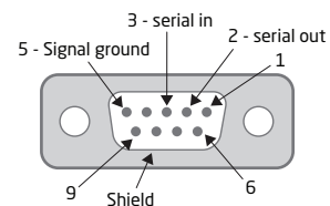
Serial: RS232 DB9 socket
